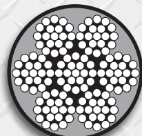
7 x 19
