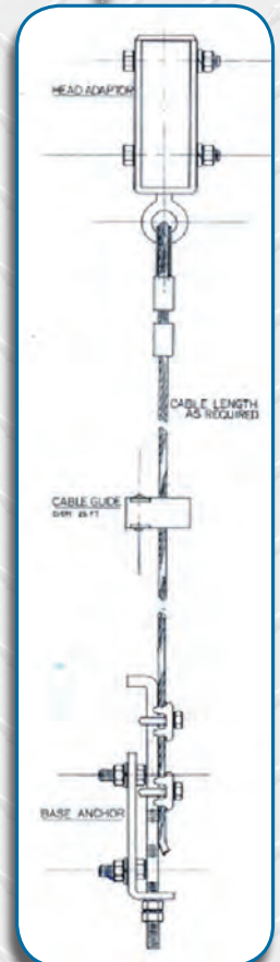
MONOPOLE SYSTEM
